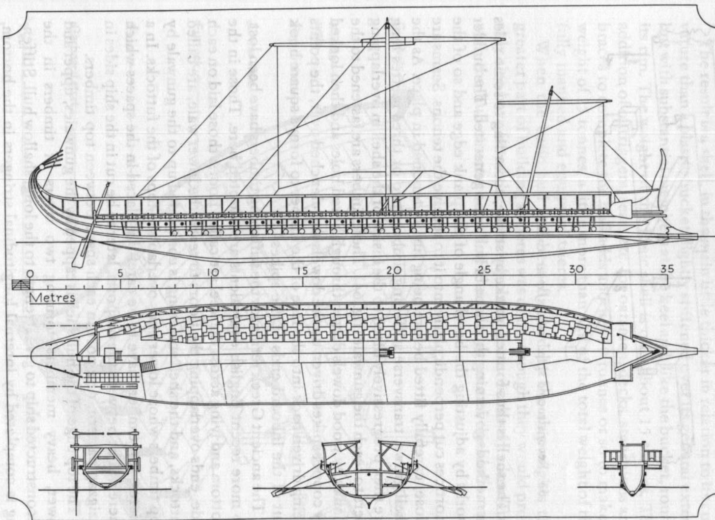
62. General arrangement of reconstructed ship.
